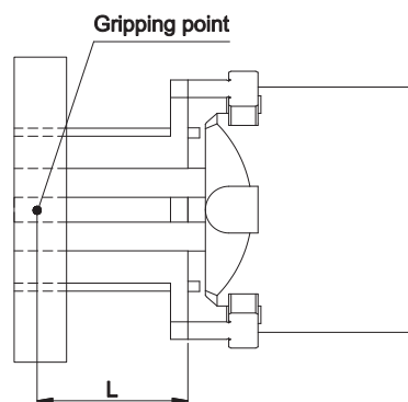
In-side clamp
